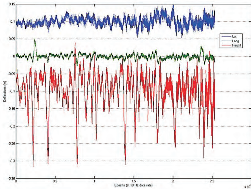
Fig. 37. The Lateral, Longitudinal and Vertical displacements at location B over a 40 minute period on the Seven Suspension Bridge. If this data is looked at in more detail, Figure 38, it can be seen that there is a clear sinusoidal pattern in the vertical displacement.
