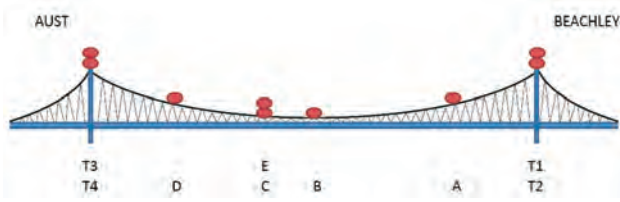
Fig. 34. The locations of the 9 GPS/GNSS receivers upon the Severn Bridge.
