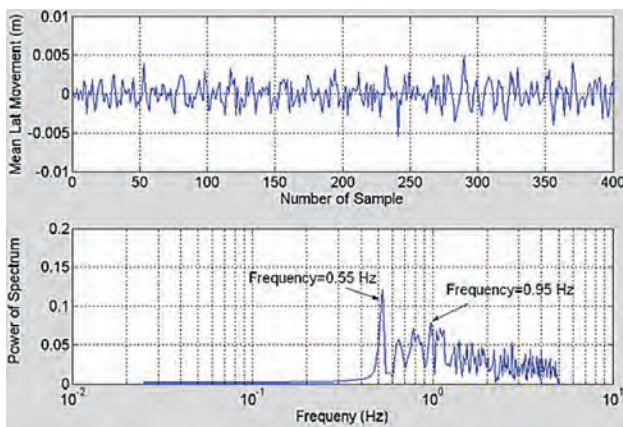
Fig. 15. Lateral dynamics on the Millennium Bridge's midspan [28].
