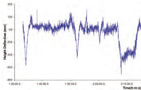
Fig. 5. Height deflection of main span east mid span on the Humber Bridge [23].
