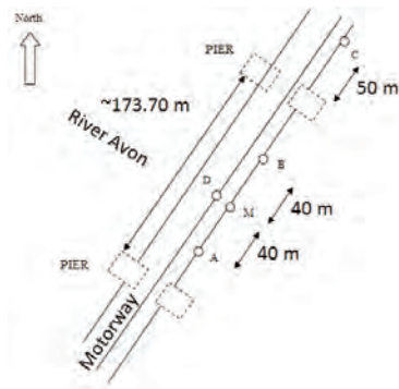
Fig. 27. An illustration of the Avonmouth M5 Motorway Viaduct and the location of the GPS antennas.
