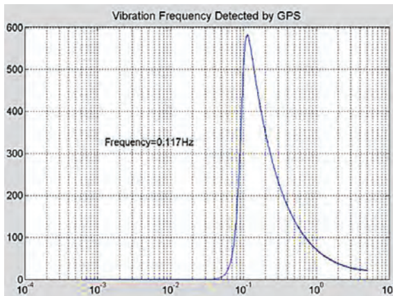
Fig. 10. The Natural Frequency of the vertical direction of the Humber Bridge obtained from the GPS data using FFT analysis in Matlab [28].
