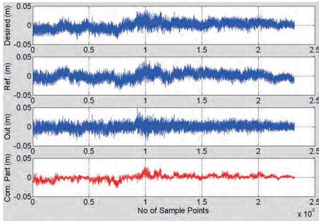
Fig. 19. Multipath analysis of the GPS data through the use of Adaptive Filtering.
