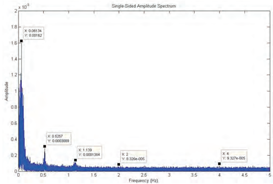
Fig. 33. The Amplitude Spectrum analysis of location M on the 29th November 2007, the Avonmouth viaduct.
