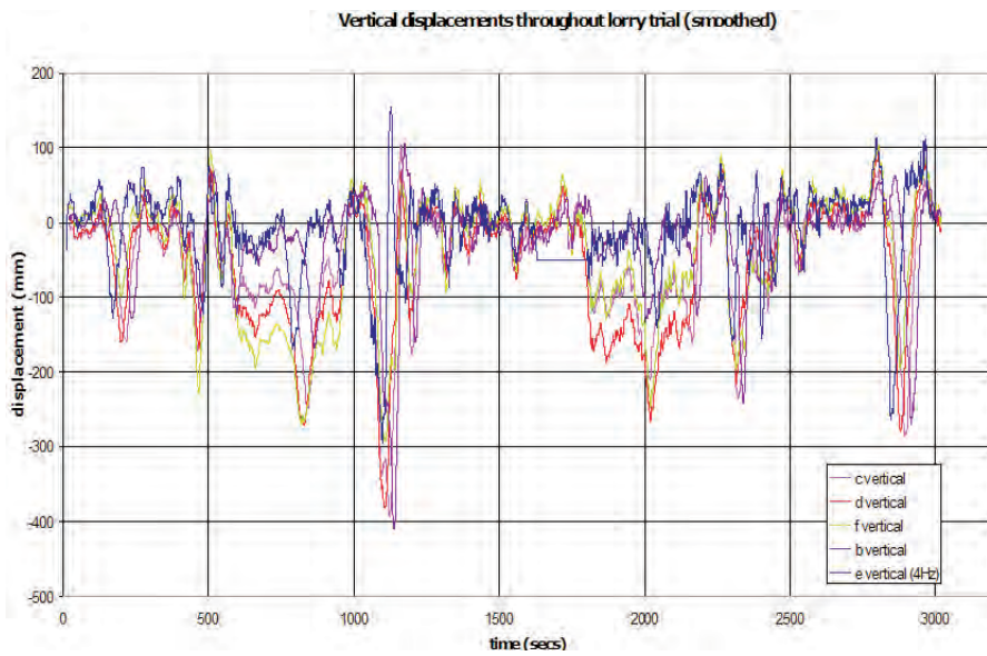
Fig. 23. Vertical displacements during the Two HGV trials on the Forth Road Bridge [30].
