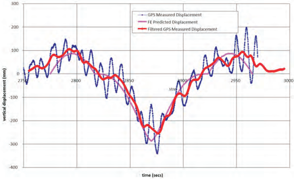
Fig. 25. Comparison between the GPS vertical displacements at location D with the FEM on the Forth Road Bridge [30].
