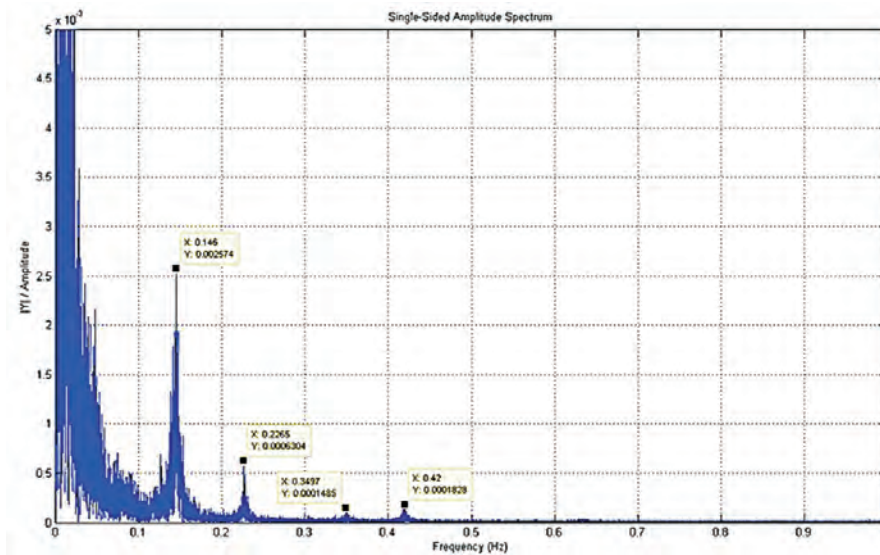
Fig. 41. FFT analysis in the vertical direction at location B on the Seven Suspension Bridge.
