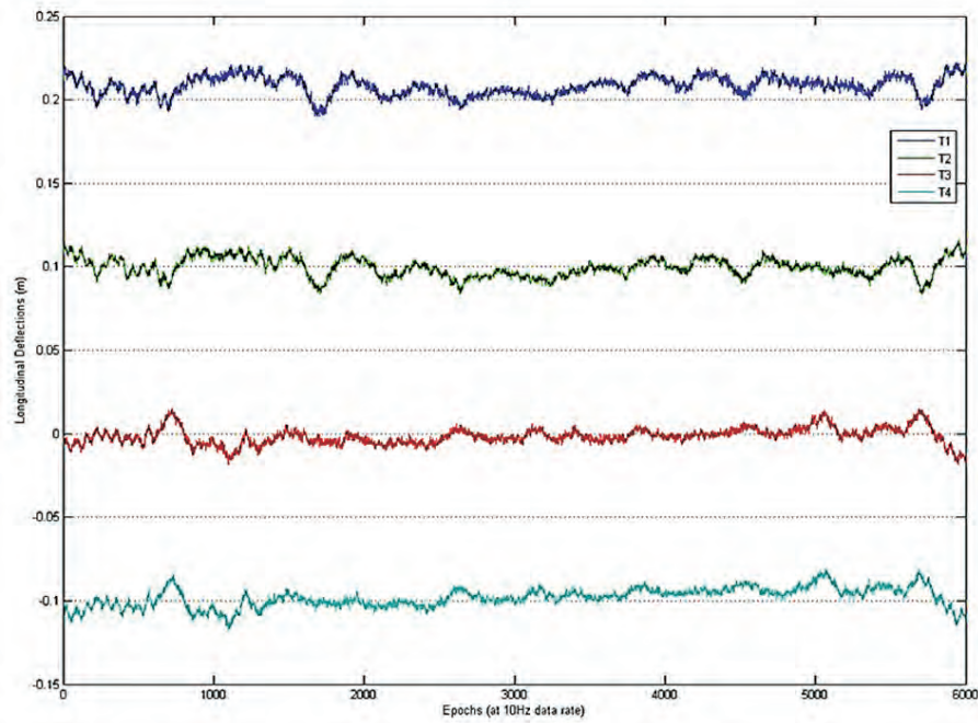
Fig. 40. The longitudinal displacements of the four tower locations over a 10 minute period on the Seven Suspension Bridge.
