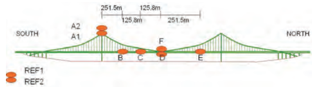
Fig. 22. The location of the GPS antennas upon the Forth Road Bridge [30].
