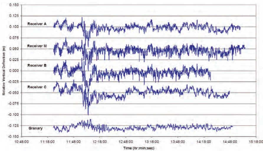
Fig. 31. The vertical movements at the granary location as well as the viaduct locations A, M, B and C over a 3.5 hour period on the Avonmouth viaduct [21].
