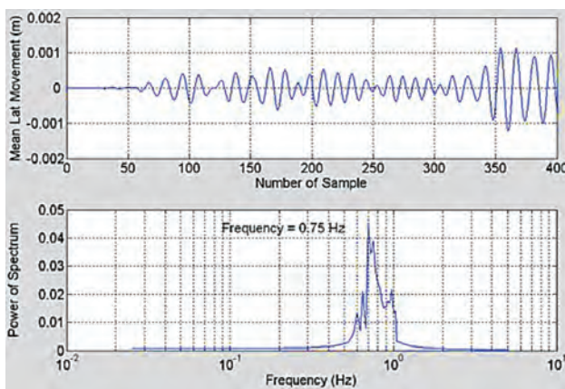
Fig. 16. Lateral dynamics on the Millennium Bridge's south span [28].
