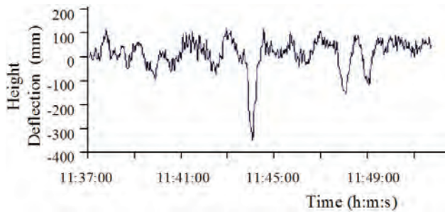
Fig. 3. Humber Bridge RTK Results in the Height Direction, 7 March 1996 [2].
