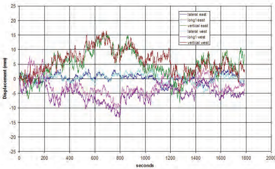
Fig. 17. The two Millennium Bridge’s midspan GPS receivers’ deflections having had a 20s moving average filter applied [26].
