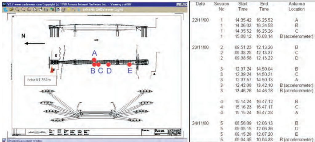
Fig. 14. The locations and times of locations of the 3 GPS receivers at the 5 monitoring points on the Millennium Bridge [26].
