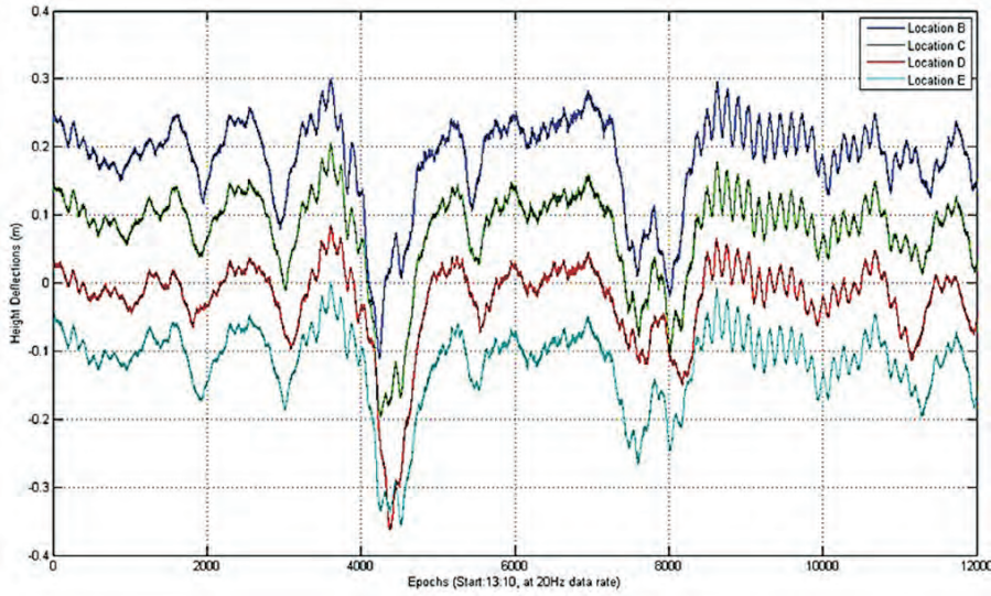
Fig. 39. The vertical displacements at the 4 Bridge deck locations over a 10 minute period on the Seven Suspension Bridge.
