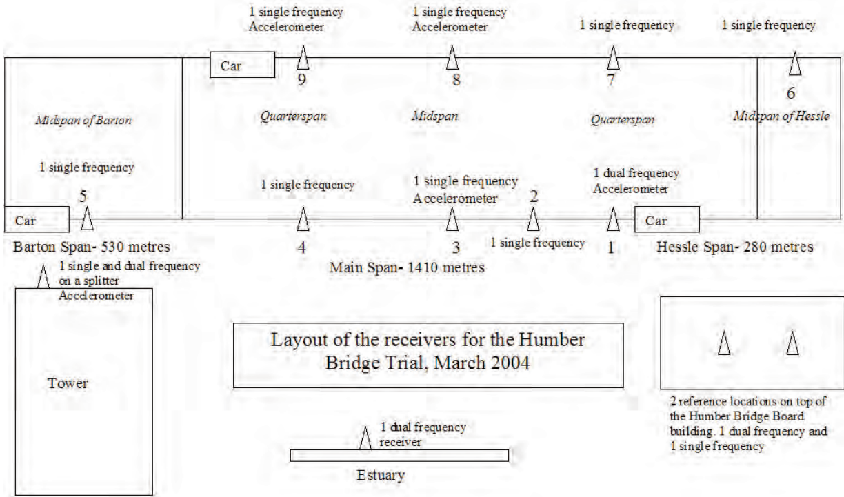
Fig. 7. The Locations of the various instruments during the field trials on the 1-4 March 2004 on the Humber Bridge [27].
