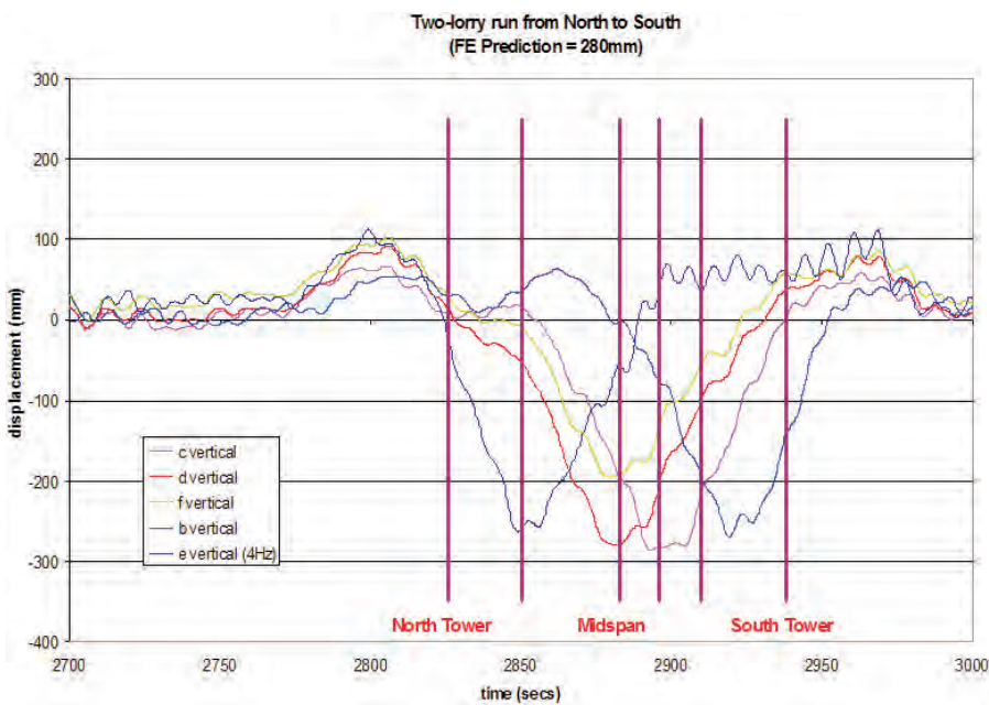
Fig. 24. Vertical displacement during the Two HGV trials with the two HGVs travelling side by side from north to south on the Forth Road Bridge [30].
