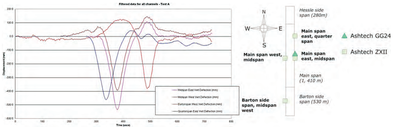
Fig. 4. Height deflections at the various GPS stations during the passage of the four HGVs over the Humber Bridge.
