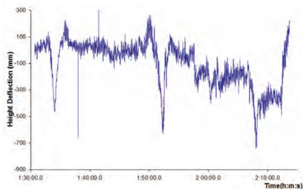
Fig. 6. Height deflection of main span west mid span on the Humber Bridge [23].
