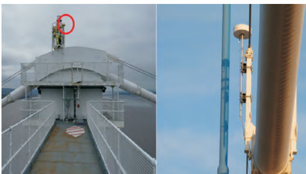
Fig. 36. A Leica choke ring AT504 antenna placed at location T2 (right), and a Leica AT503 lightweight choke ring antenna placed at location C (right) on the Severn Suspension Bridge.
