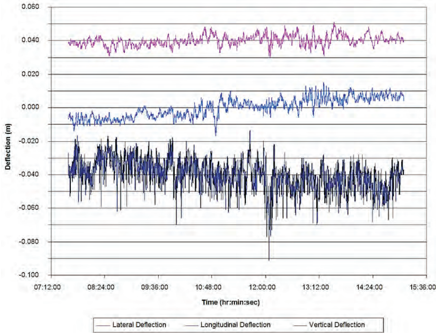
Fig. 30. Lateral, longitudinal and vertical movements of location M on the 30 November 2007, the Avonmouth viaduct.
