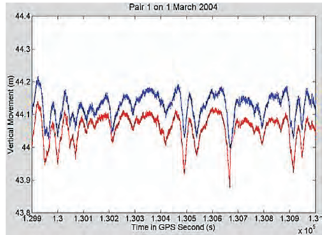
Fig. 9. Two GPS antenna results from locations on opposite sides of the Humber Bridge, showing the effect of twisting on the Bridge deck [28].
