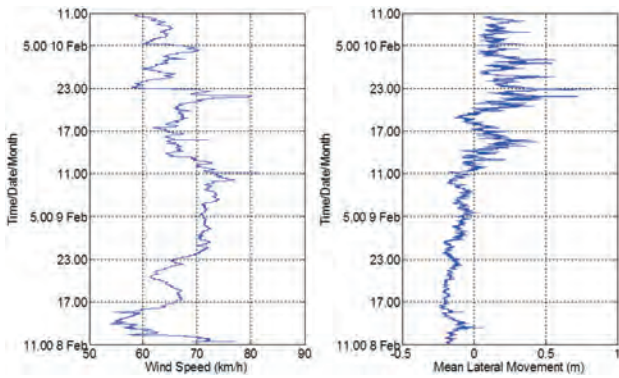
Fig. 26. Comparison between the GPS derived lateral movements on the Bridge and the wind speed at location F [30].
